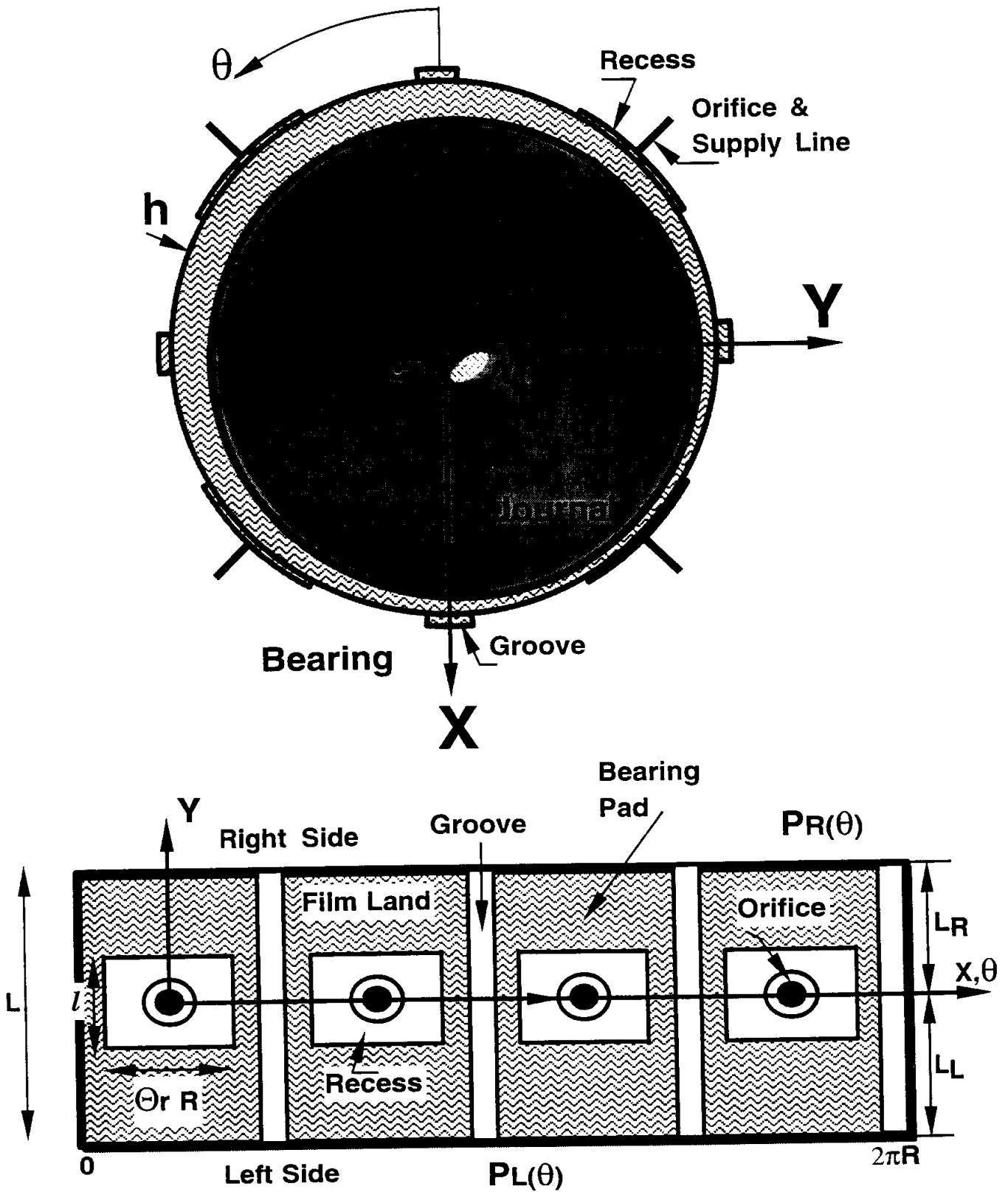
Fig.1 Geometry of Hydrostatic Pad Bearing
