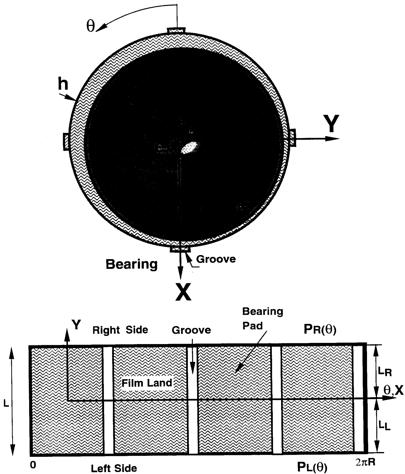
Fig. 3 Geometry of Fixed Arc Pad Bearing
