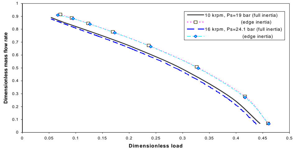
Dual Use 6-pocket HTB for R134a compressor, T_s=38\text{ C}
