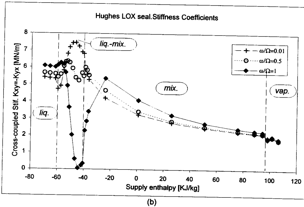
Figure 19. Variation of dynamic stiffness with supply enthalpy for different excitation frequencies. (a) Direct stiffness, K_{xx} . (b) Cross-coupled stiffness, K_{xy} .
