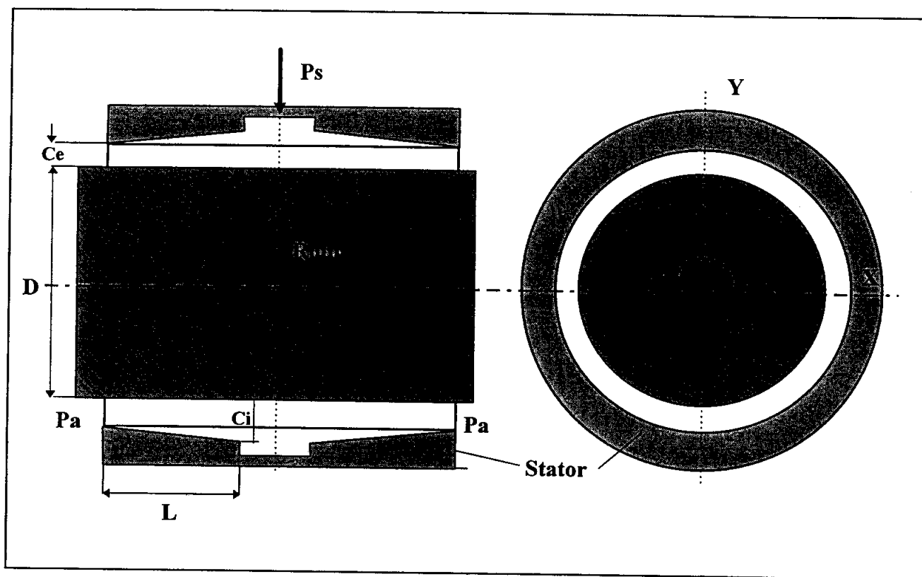
Figure 10. Schematic view of the seal geometry for the HPOTP-SSME seal example.
