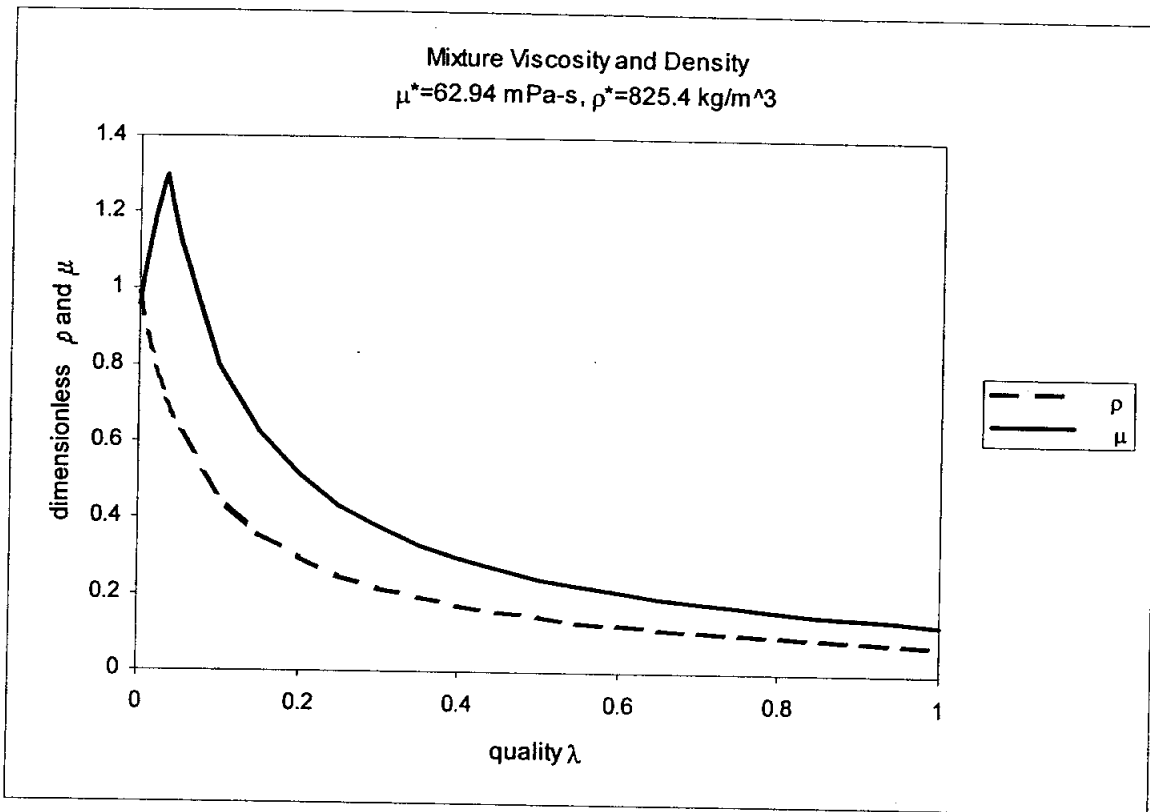
Figure 4. Variation of dimensionless mixture viscosity and density with quality for liquid oxygen (LOX) at P=1.8 MPa ( T_{\text{sat}}=130.58 °K).
