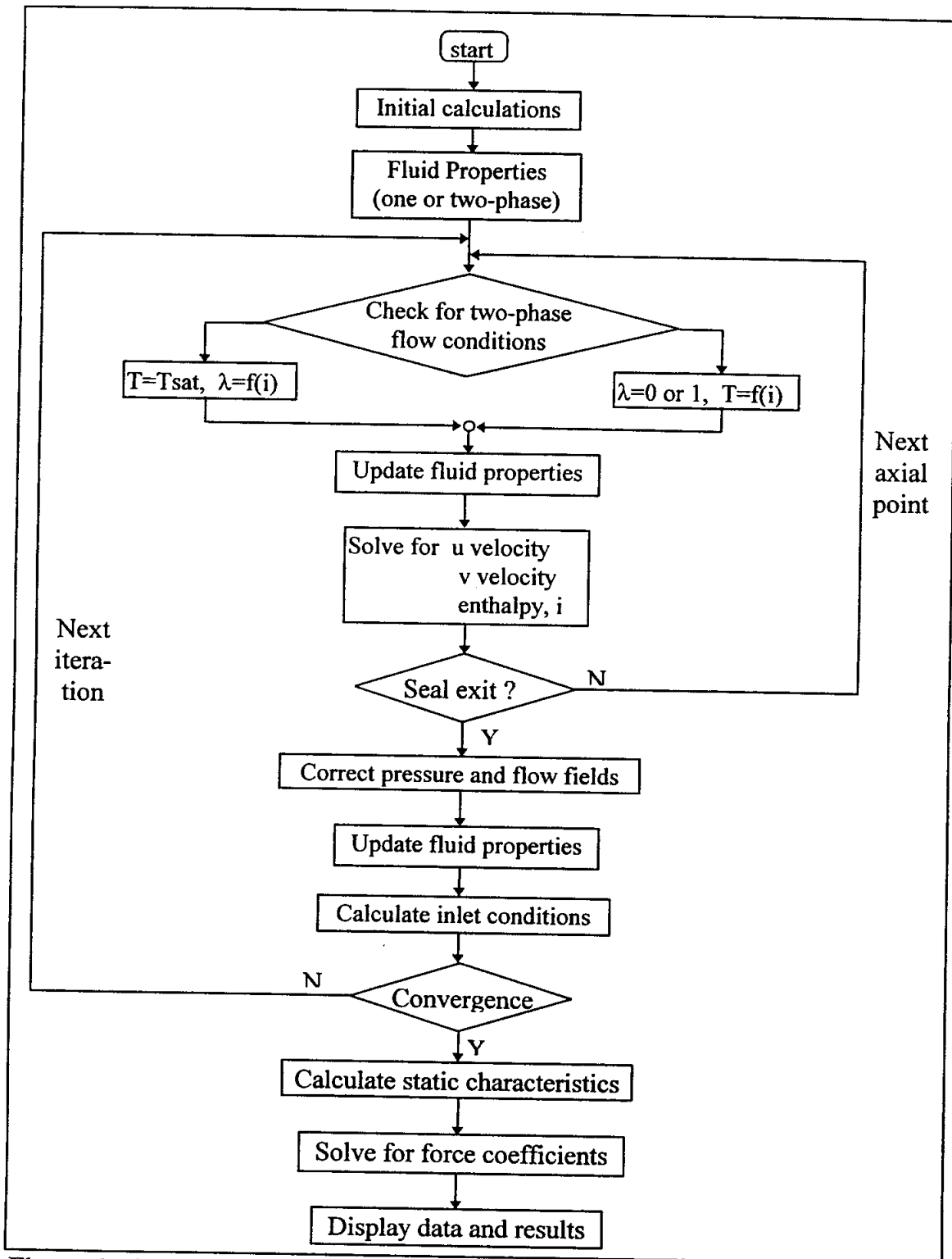
Figure 6. Flow chart illustrating numerical algorithm.
