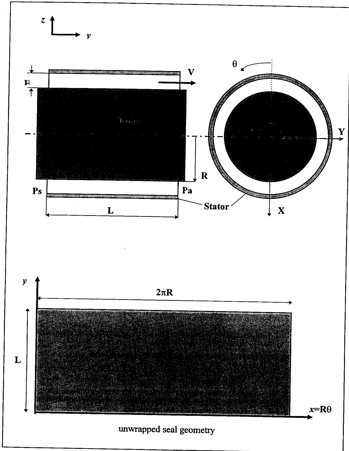
Figure 3. Schematic annular pressure seal geometry and coordinate system.
