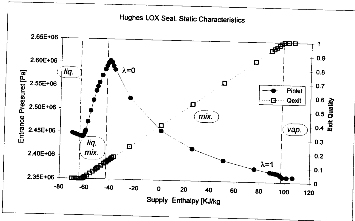
Figure 17. Leakage, torque, entrance pressure and exit quality for different supply enthalpies.
