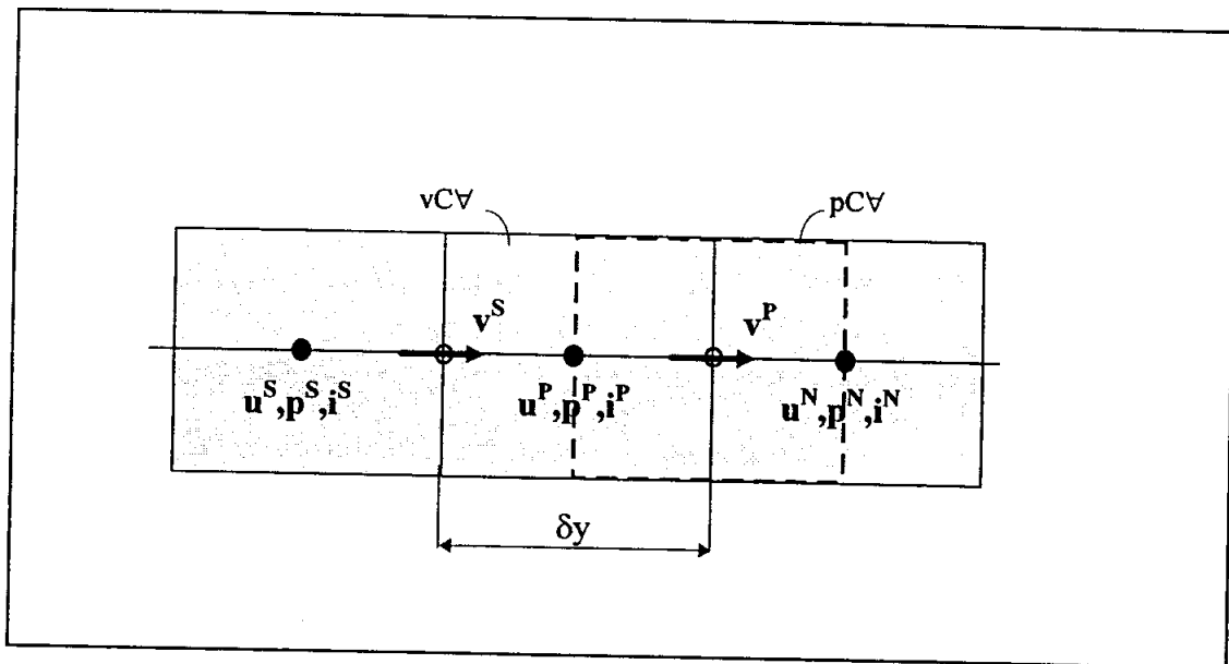
Figure 5. Schematic diagram of staggered grid sand control volumes used.
