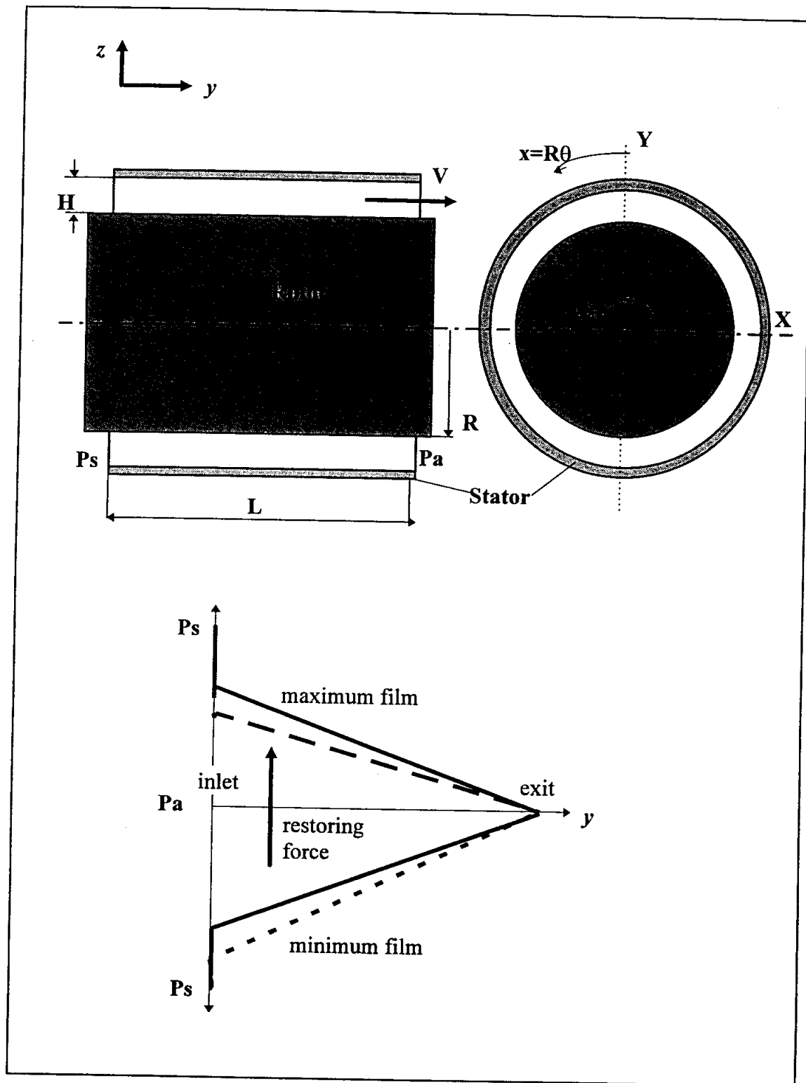
Figure 1. Seal geometry and restoring fluid forces.
